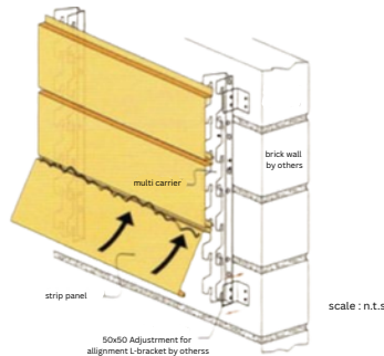
Typical installation plan for strip ceiling with Multi Carrier
