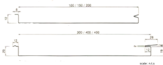
Typical Detail at Bottom STRIP FACADES to floor
