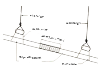
Typical Detail joint using Panel Joint
