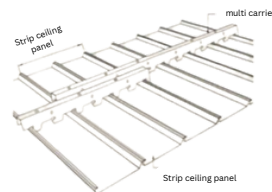
Multi Carrier joint detail
