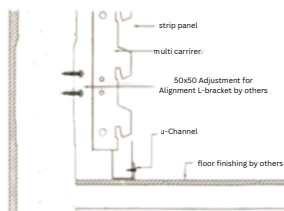
Typical Detail at Bottom STRIP FACADES to floor
