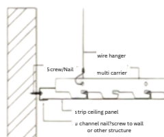
Typical Gable End of ceiling type
