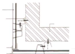
Typical Detail at Bottom STRIP FACADES
